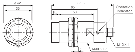
●PRCML30-15D□ / PRCML30-15A□
